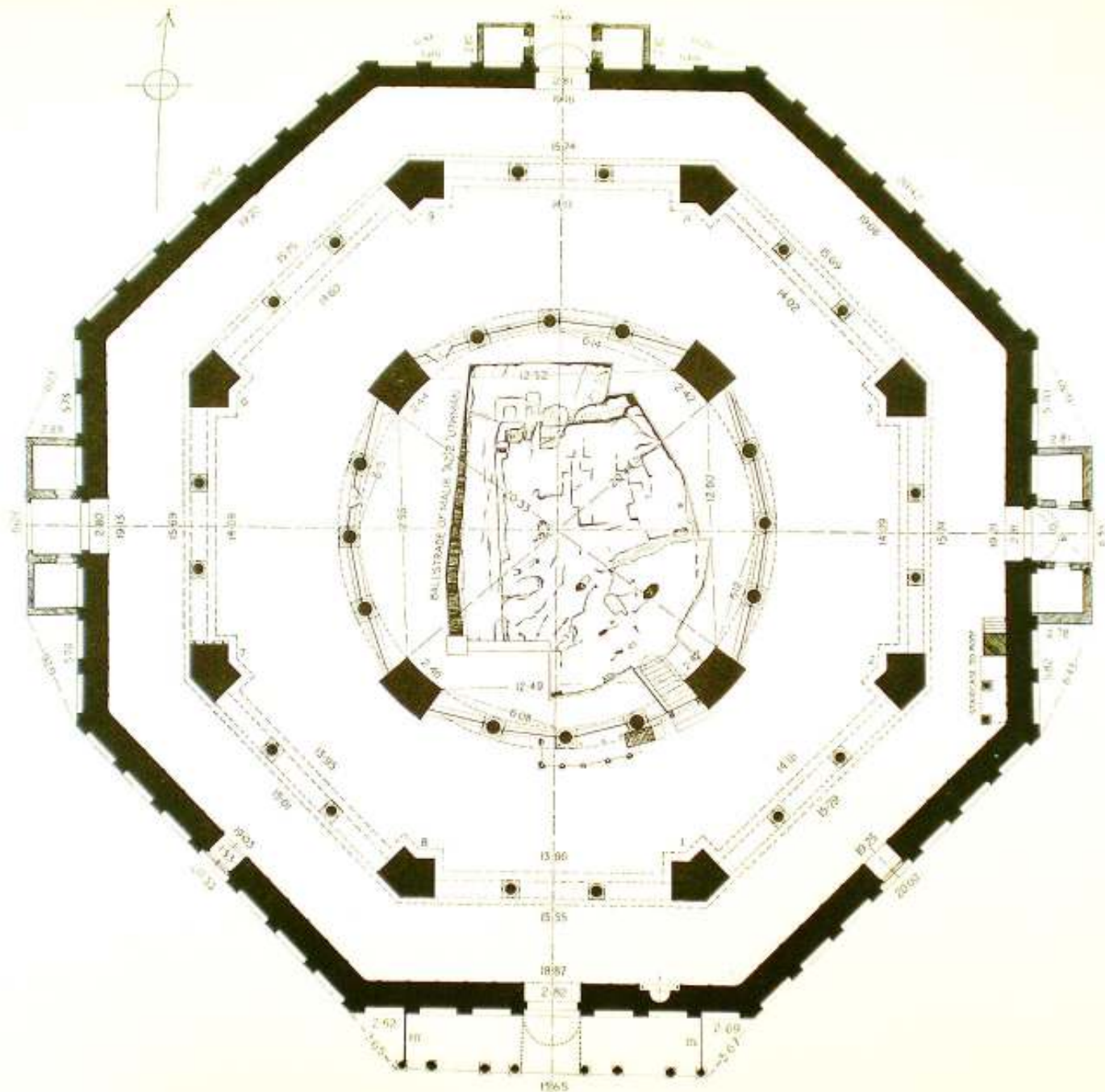
FIG. 21. JERUSALEM: The Dome of the Rock, or Qubbat as-Sakhra, plan.
